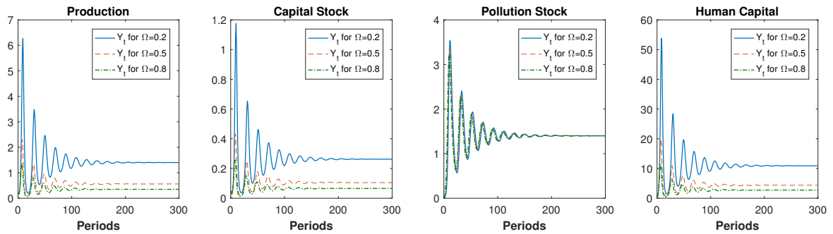
Figure 10: The effect of \Omega on the convergence, for a = 0.5
